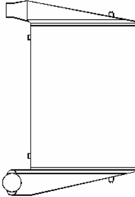
Dimensional Data: MAS255C
