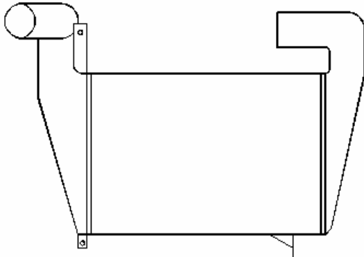
Dimensional Data: MAS255A
