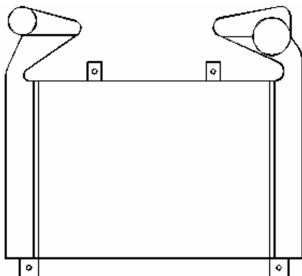
Dimensional Data: MK18E4
