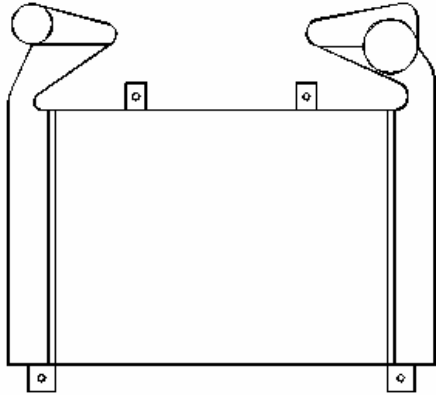
Dimensional Data: MK18E5
