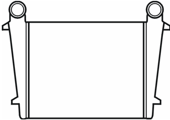
Dimensional Data: MK16B
